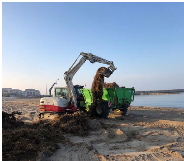
Figure 4 Mechanical beach wrack collection (© Hanseatische Umwelt CAM GmbH)
